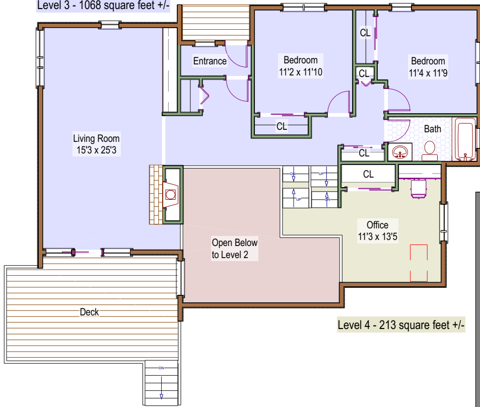
Level 3 - 1068 square feet +/-
