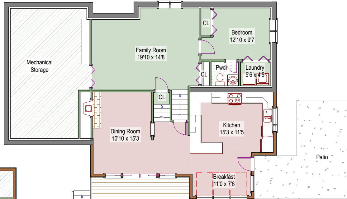
Level 2 - 619 square feet +/-
